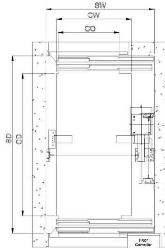
1000 kg / 2 Side Opening Doors
