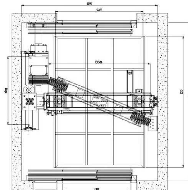
GIGAS 2500 kg / 2 Side Opening Doors
